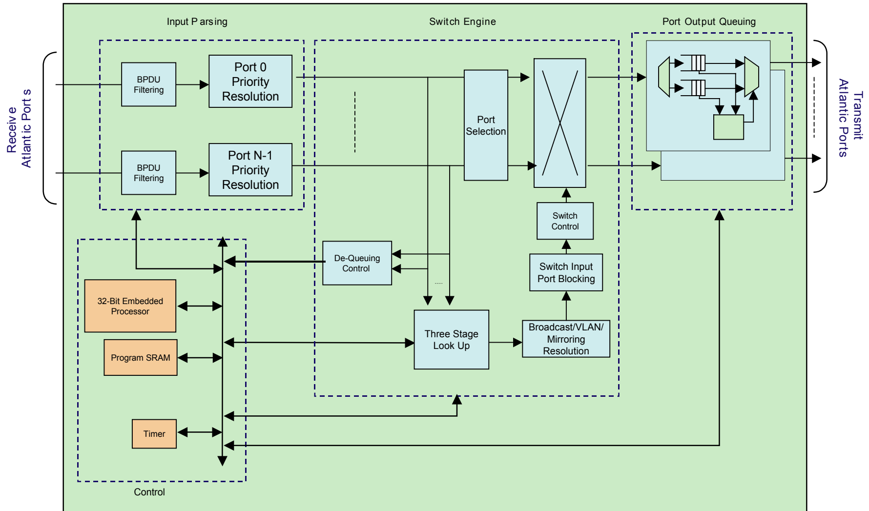
Figure 1: Ethernet Layer 2 Switch Block Diagram
