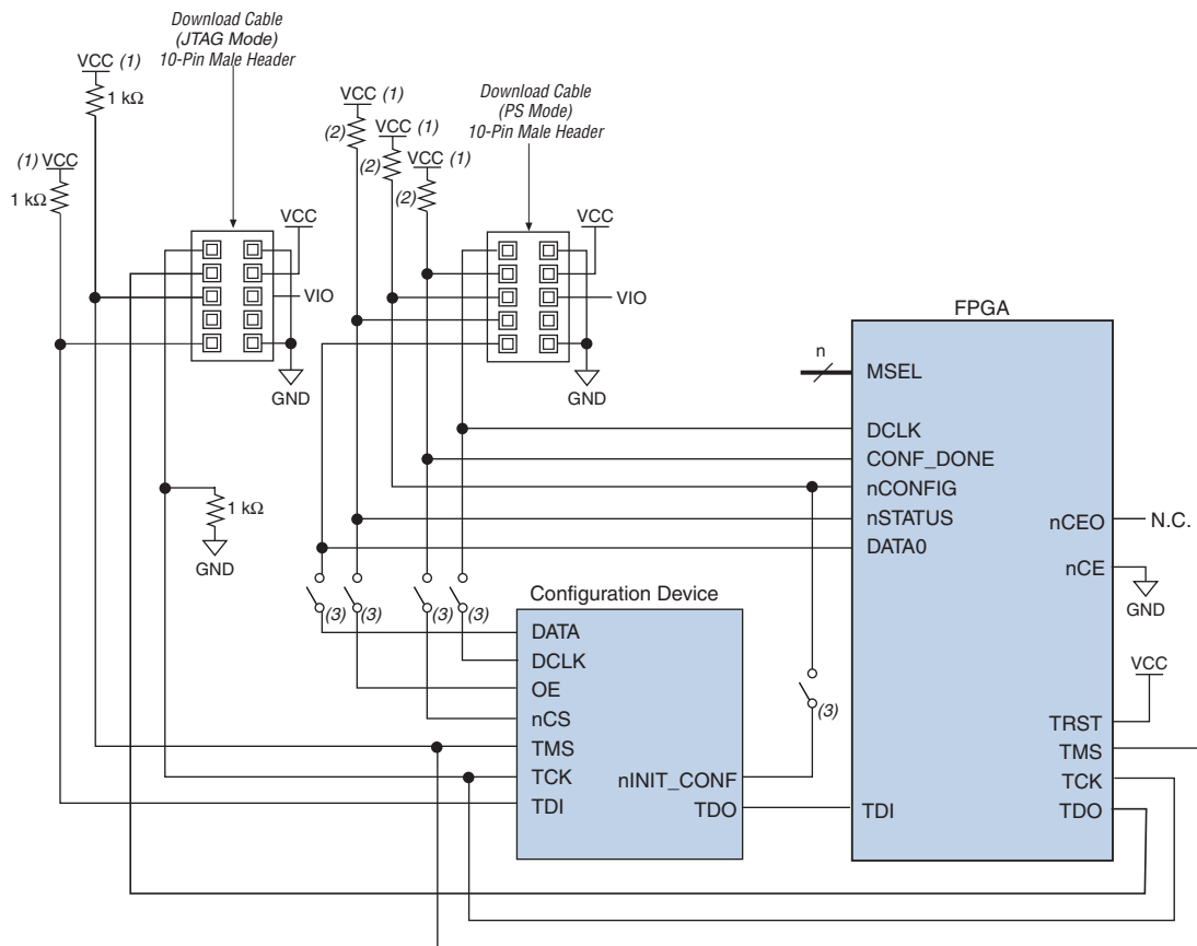
Figure 9-4. Combining JTAG Programming of Configuration Device and FPGA with PS Configuration of FPGA Using a Configuration Device and Download Cable
