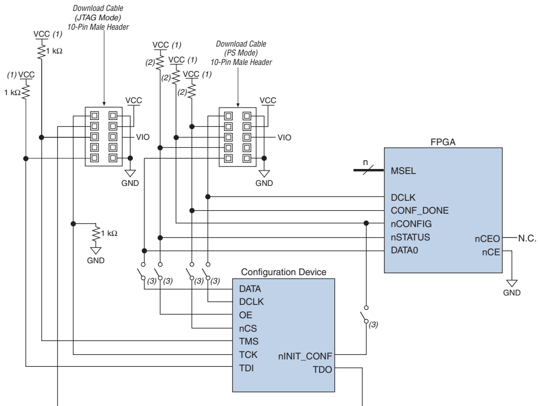
Figure 9-3. JTAG Programming of Configuration Device with PS Configuration of FPGA Using a Configuration Device and Download Cable
