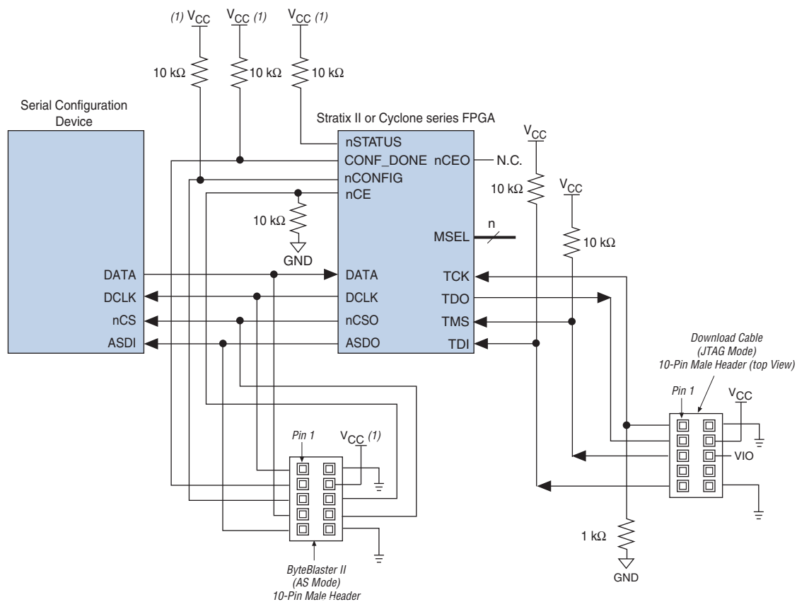
Figure 9-5. Combining JTAG Programming of Configuration Device and FPGA with AS Configuration of FPGA Using a Configuration Device and Download Cable
