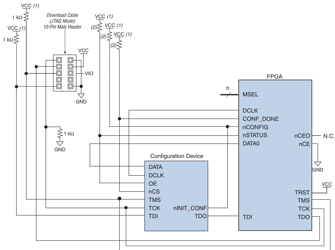
Figure 9-2. JTAG Programming of Configuration Device and FPGA with PS Configuration of FPGA Using a Configuration Device
